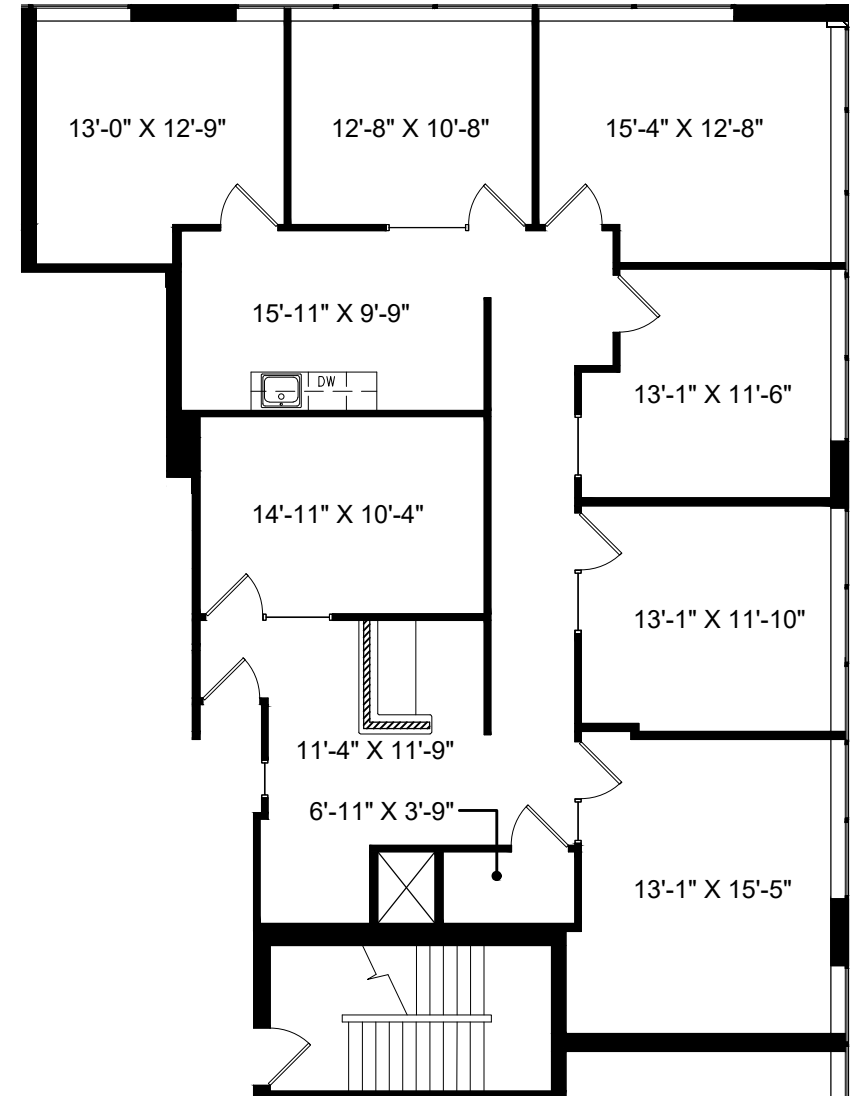
SUITE 208 - 2,197 RSF NOT TO SCALE
